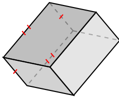
prisma rectangular
