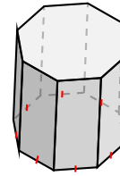
prisma octagonal
