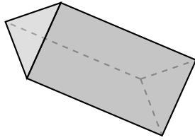
prisma triangular
