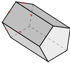
prisma pentagonal
