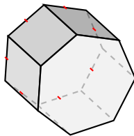
prisma heptagonal
