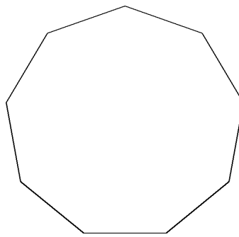
Eneágono Regular
